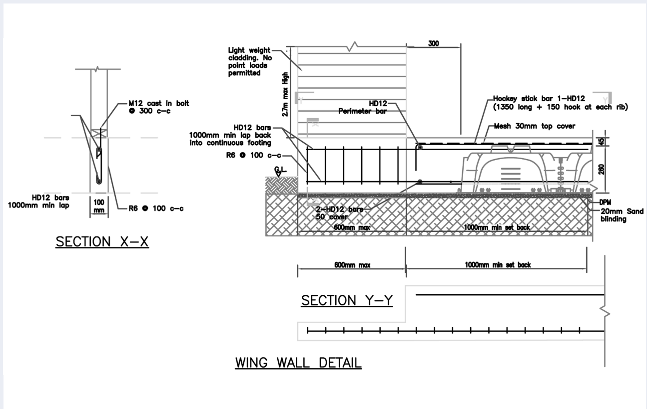
FIGURE 34 - Qpod wingwall detail
