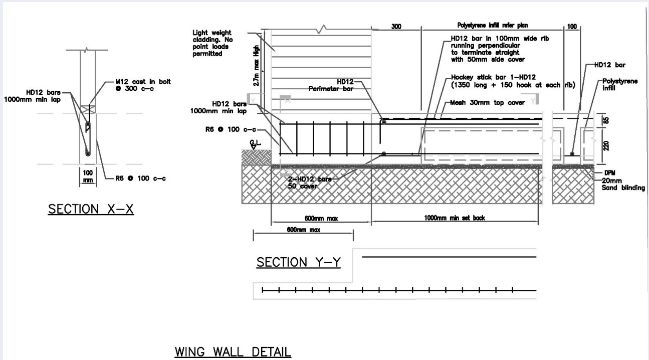
FIGURE 22 - Wingwall detail
