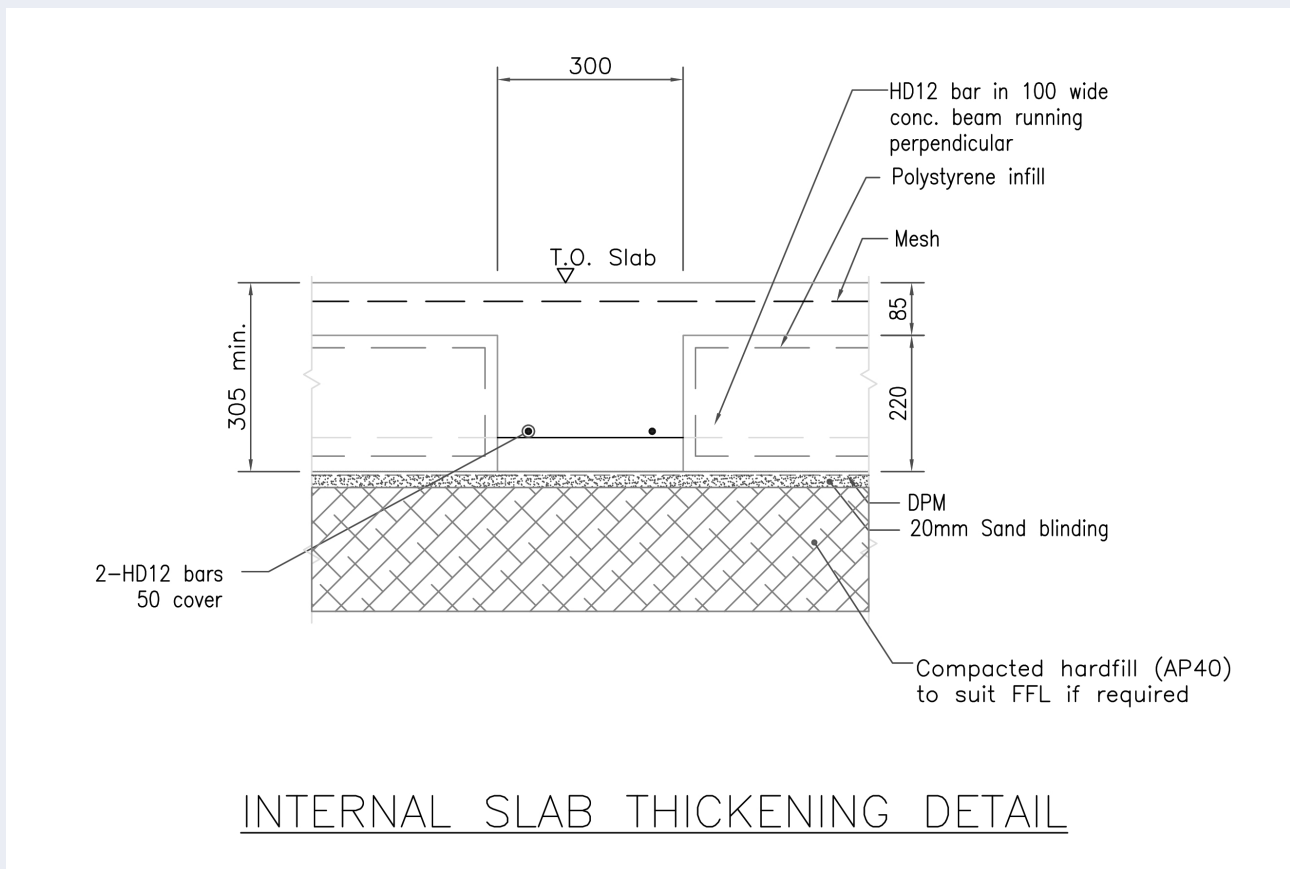
FIGURE 18 - Internal slab thickening
