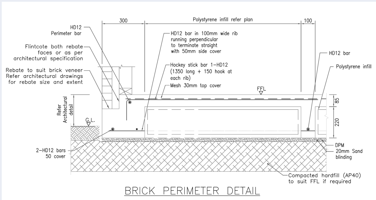
FIGURE 17 - Brick Rebate detail
