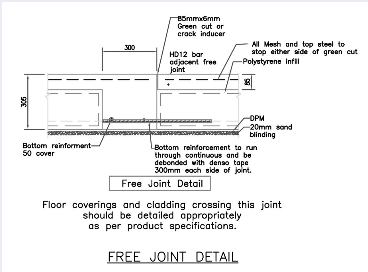
FIGURE 21 - Free Joint
