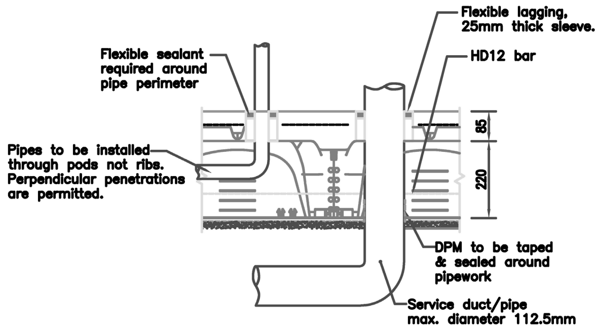
TYPICAL SERVICES PENETRATIONS DETAIL
