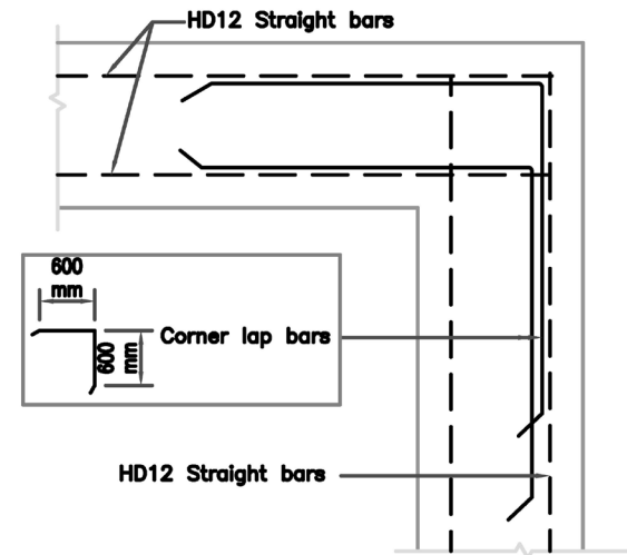
Typical Corner Laps Detail Scale 1:20
