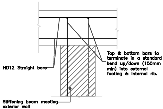
Typical Stiffening Detail
