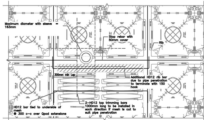
TYPICAL SERVICES THROUGH RIBS
