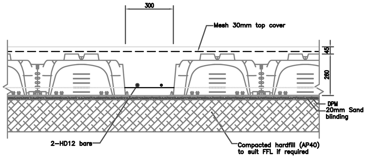
INTERNAL SLAB THICKENING DETAIL
