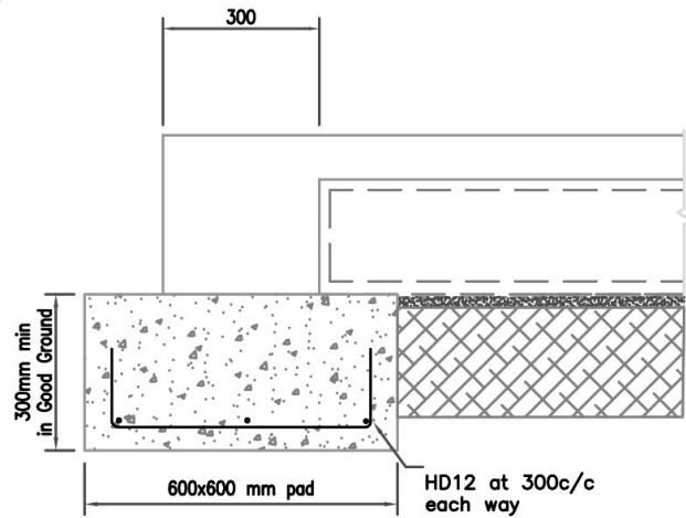
SECTION X-X
