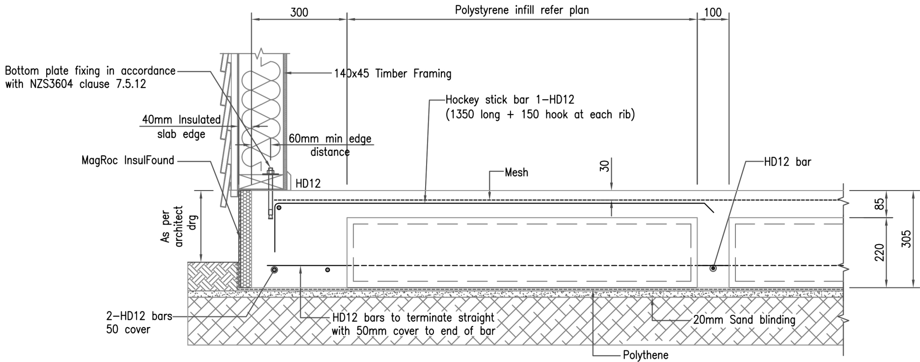
LIGHT WEIGHT CLADDING ALLIED SUPERSLAB WARMEDGE DETAIL
